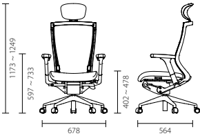
TN500HDAPU with adjustable neckrest and headrest / polished aluminum with powder coating base on the basic type
